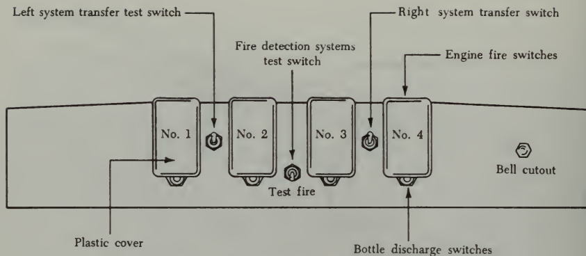
FIGURE 9-16. Fire detection system and fire switches.
